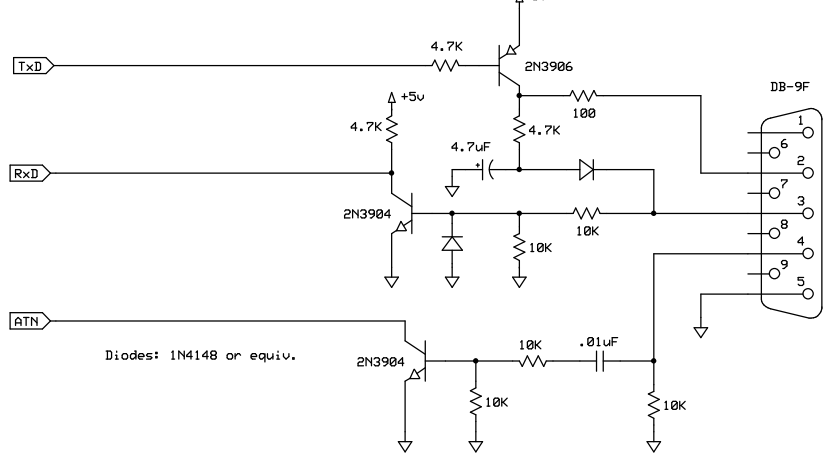
Suggested Serial Interface #3
