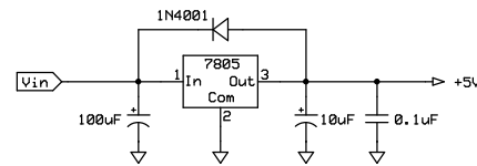
Voltage Regulator
